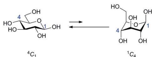
Fig. 2 \beta -D-glucopyranose conformations.
