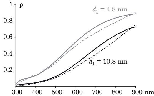
Figure 7: Measured (solid line) and predicted (dashed line) reflectance of the coated glass plates (Samples B) in front of a Lambertian white tile. Measurements are based on a 45^\circ:0^\circ geometry.
