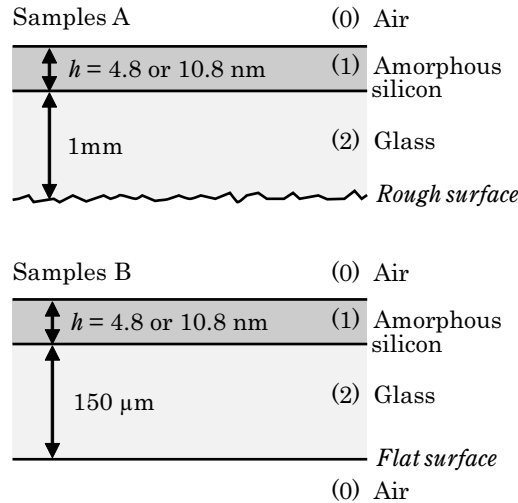
Figure 2: Description of the multilayer samples A and B.
