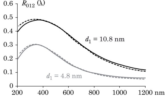
Figure 4: Predicted (dashed line) and measured (solid line) spectral reflectances of silicon coatings on 1mm thick glass plates (Samples A) at 7^\circ from the normal.
