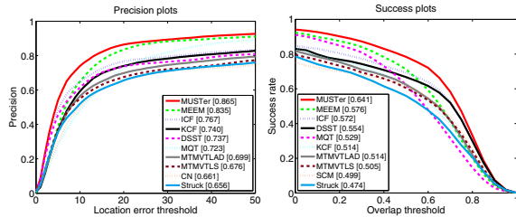
Figure 4. Quantitative comparison in CVPR2013 OOTB. The performance score for each tracker is shown in the legend. For each figure, only the top 10 trackers are presented.
