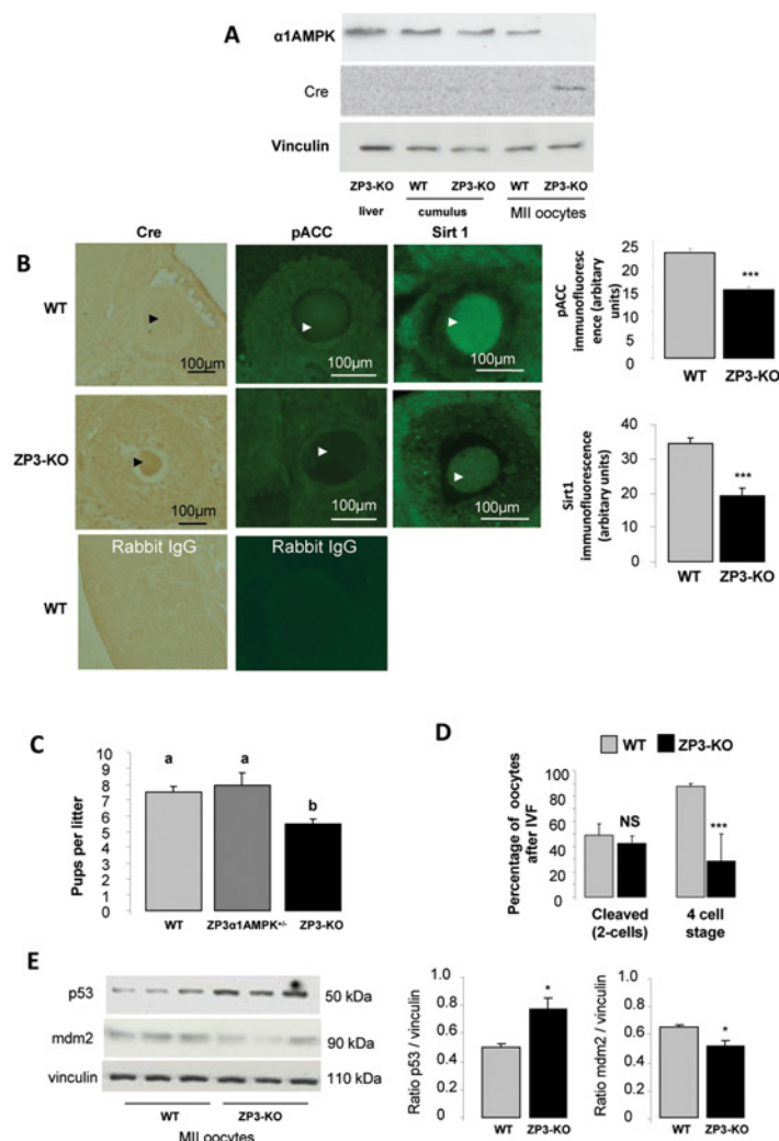
Fig 1. \alpha 1 AMPK inactivation in oocyte. (A) Western blot analysis of the \alpha 1 AMPK subunit and Cre recombinase in metaphase II (MII) oocytes, cumulus cells and liver retrieved from wild-type and ZP3-KO mice after superovulation (B) Conditional invalidation of \alpha 1 AMPK subunit in the oocyte. Cre expression was localised by immunohistochemistry, and phospho-ACC, and Sirt1, two AMPK substrates, by immunofluorescence in WT and ZP3-KO ovary sections. Arrows show the oocyte (C) Fertility analysis of WT (genotype AMPK \alpha 1^{lox/lox} ), heterozygous (genotype ZP3-Cre, AMPK \alpha 1^{+/-} ), and ZP3-KO (genotype ZP3-Cre, AMPK \alpha 1^{-/-} ) female mice were mated with wild-type males. (D) Percentage of oocytes cleaved after in vitro fertilization with wild type semen and percentage of cleaved oocytes to reach a 4-cell stage embryo. (E) Western blot analysis of p53 and mdm2 protein levels in MII oocytes of WT and ZP3-KO mice. *, P < 0.05 ***, P < 0.001 . a, b Values with different letters differ significantly ( P < 0.05 )
