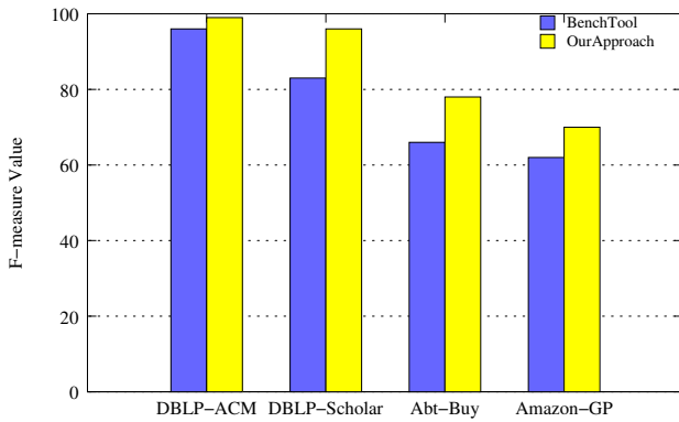
Figure 2: Results of BenchTool and our approach in terms of F-measure for the 4 datasets.
