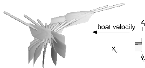
Fig. 2. Kinematics of the blade for the F001 experiment in the water frame of reference (with subscript 0).
