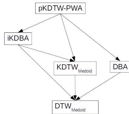
Fig. 8. Dominance graph for the five tested algorithms, according to the significance relation corresponding to Table 3 with a P-value threshold set to .05.
