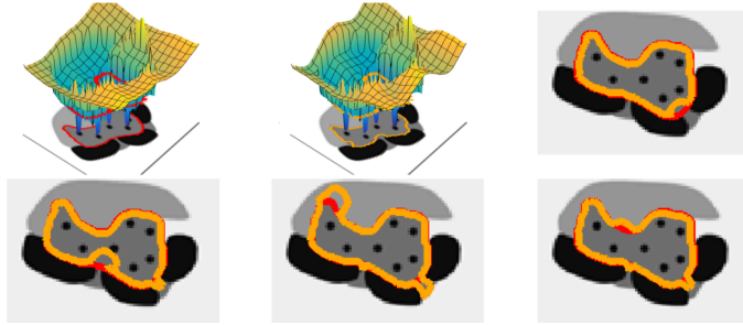
Fig. 2: (Top Left) Mean of the GP \mu ; (Top Middle) Sample of the level function \varphi(\mathbf{x}) drawn from \mathcal{GP}(\mu, \Sigma) ; (Others) GPSSSI samples. The ground truth is outlined in red, the GPSSSI samples are outlined in orange.
