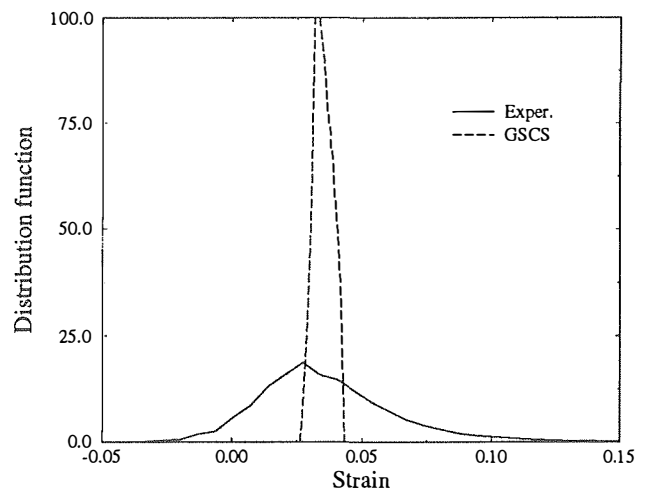
FIG 4. Strain distribution function in the iron at 5% global strain
