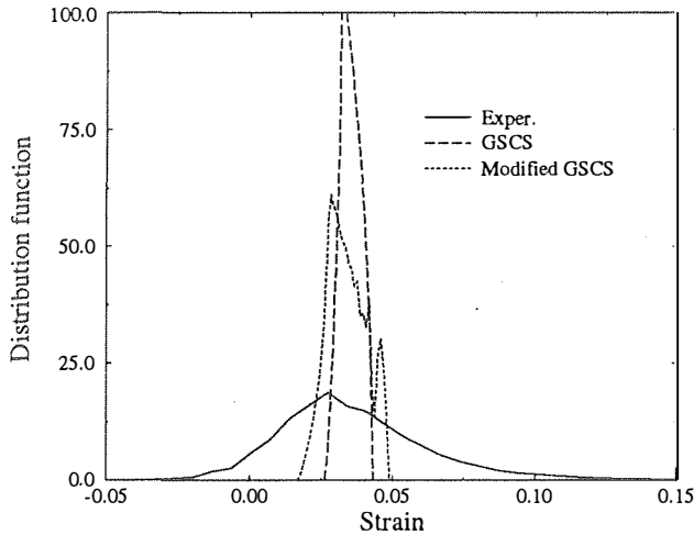
FIG 14. New non-linear extension (iron at 5% global strain)
