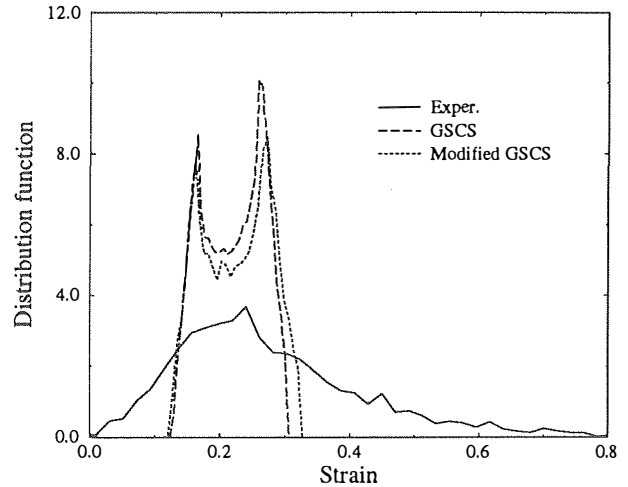
FIG 15. New non-linear extension (silver at 15% global strain)
