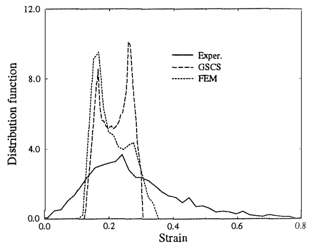
FIG 19. FEM results (silver at 15% global strain)
