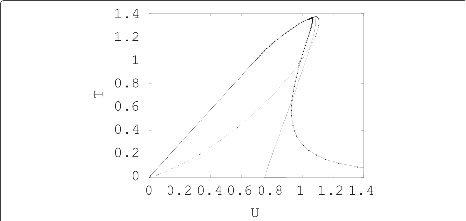
Figure 8 Force-displacement curves for n = 1 (small dots), n = 2 (solid line), n = 3 (big dots).
