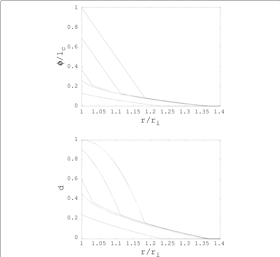
Figure 7 Distributions of \phi/l_c (top figure) and damage (bottom figure) for different loadings. Details on the curves in each plot from bottom to top: Bottom curve corresponds to T = 1.232 , damage evolution is purely local. The next curve is for T = 1.351 . It corresponds to the load at which \|\nabla\phi\| = 1 at r = r_i and non-locality steps in. Next curve is for T = 1.368 , it is the limit load. The load then decreases and damage evolution is purely non-local. Last two curves are for T = 1.012 and T = 0.02 , respectively. The latter case depicts the profile at complete decohesion of the fiber.
