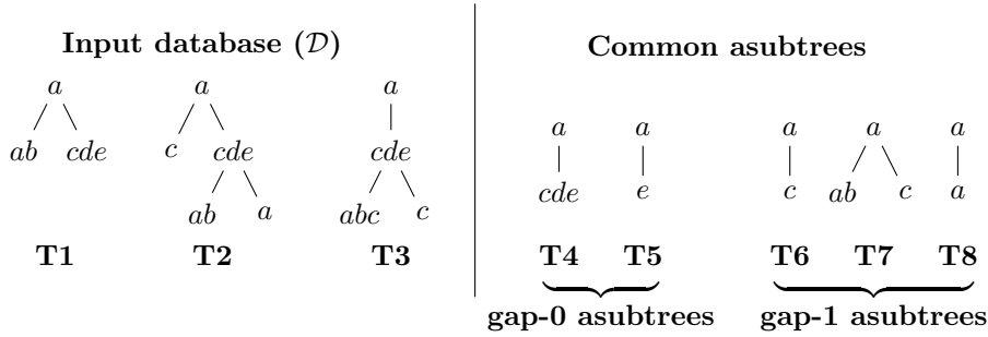
Fig. 2. Example of an atree database with some common subtrees.
