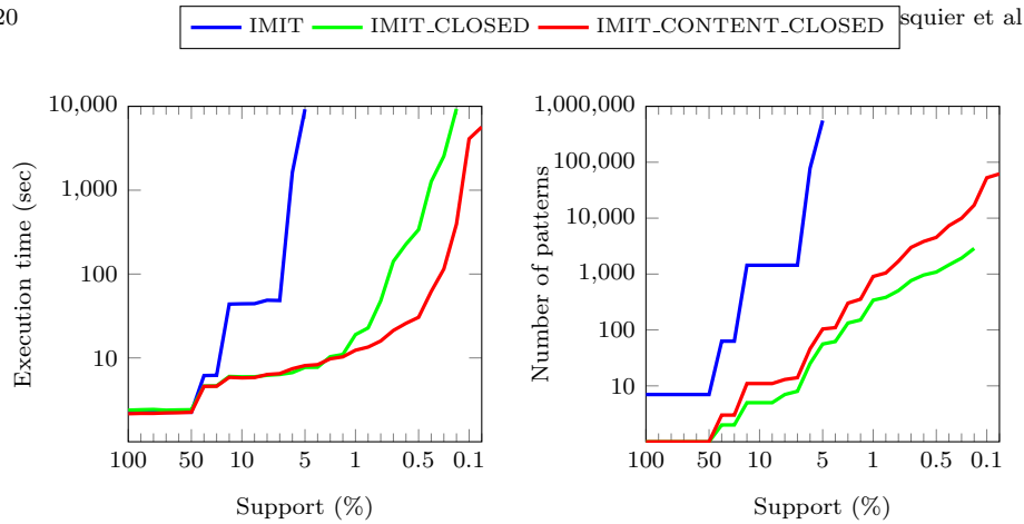
Fig. 14. Execution time (left plot) and number of patterns found (right plot) by the different versions of IMIT for mining induced unordered patterns on D10-3 dataset.
