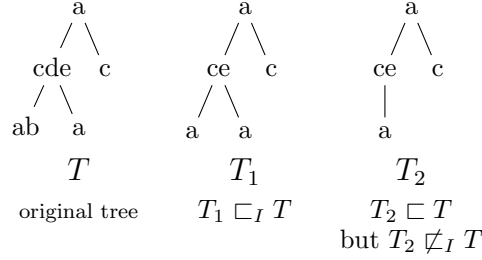
Fig. 1. Illustration of the different types of inclusion.
