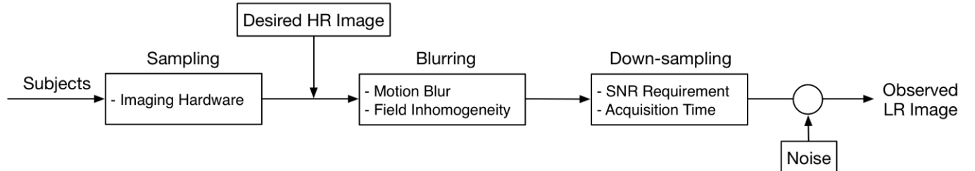
Fig. 2. Observation model in MR image acquisition process.
