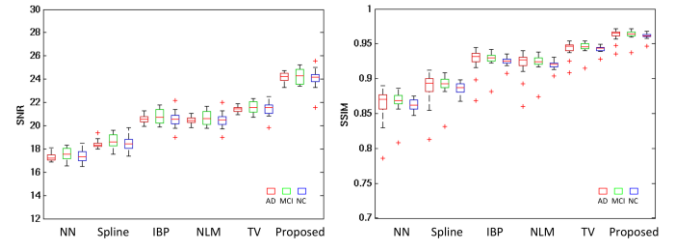
Fig. 10. Boxplot of SNR and SSIM results for recovering adult data in groups of AD, MCI, and NC.
