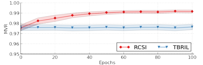
Figure 4: Performance of RCSI (and TBRIL) when the optimal policy is learned online.
