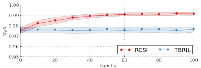
Figure 4: Performance of RCSI (and TBRIL) when the optimal policy is learned online.
