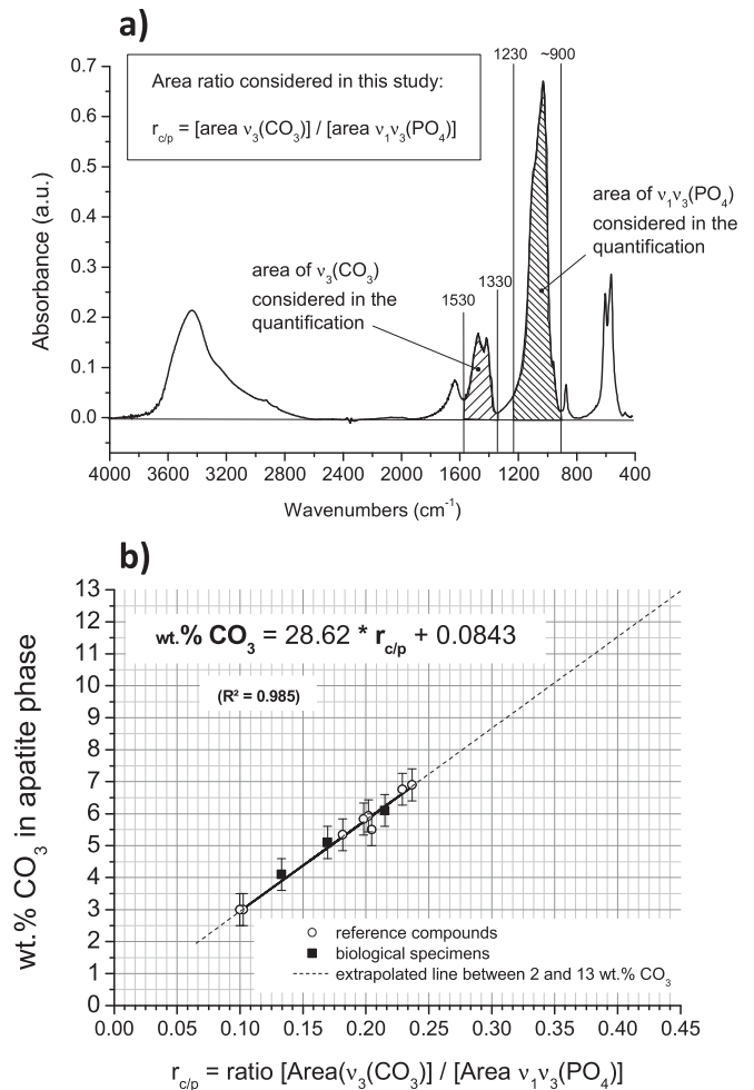
Fig. 4. FTIR methodology for carbonate quantification: a) evaluation of the ratio r_{c/p} between the integrated intensity of \nu_3(\text{CO}_3) and that of \nu_1\nu_3(\text{PO}_4) , and b) correlation between r_{c/p} and the carbonation amount (in wt.% \text{CO}_3 ) in the apatite phase of synthetic reference compounds and for three biological samples.
