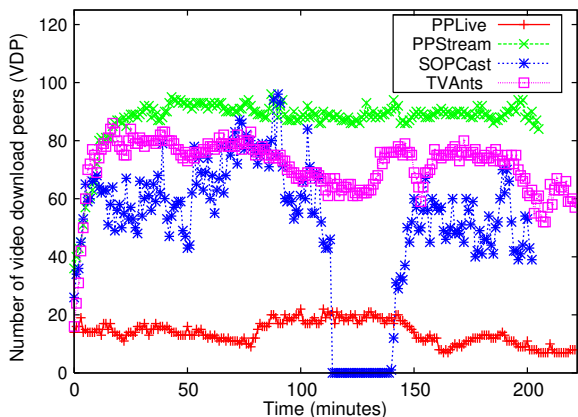
Fig. 8. Peers neighborhood for all the applications (bin duration is 60 s).
