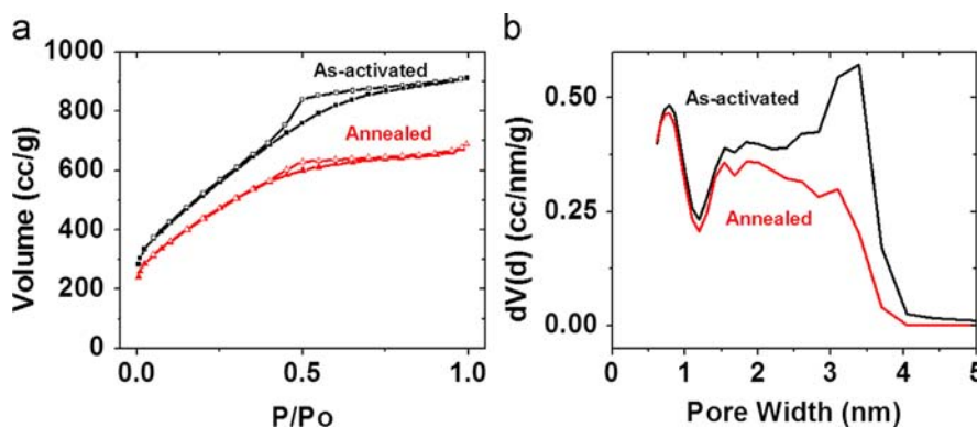
Figure 1 Nitrogen sorption isotherms (a) and corresponding pore size distributions (b) for as-activated (BET SSA 1900 \text{ m}^2/\text{g} ) and vacuum annealed a-MEGO (BET SSA 1590 \text{ m}^2/\text{g} ). After annealing, there is a decrease in the volume of small mesopores around 3 \text{ nm} , while the micropores within a-MEGO are preserved. Closed symbols in (a) represent the adsorption branch while open symbols represent the desorption branch.
