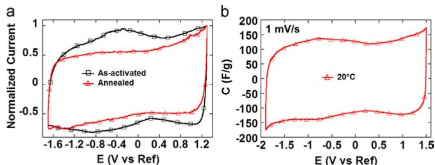
Figure 5 Cyclic voltammograms of annealed and as-activated a-MEGO electrodes in (\text{PIP}_{13}\text{-FSI})_{0.5}(\text{PYR}_{14}\text{-FSI})_{0.5} electrolyte: CVs collected at 500 mV/s at room temperature using CME (a); CV collected at 1 mV/s using a Swagelok ® cell (b).
