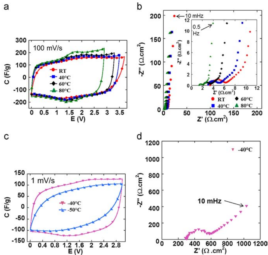
Figure 4 Electrochemical characterization of a-MEGO electrodes in (\text{PIP}_{13}\text{-FSI})_{0.5}(\text{PYR}_{14}\text{-FSI})_{0.5} electrolyte: CVs collected at 100 mV/s (a), corresponding EIS Nyquist plots (b) at room and elevated temperatures ( \text{RT} \leq T \leq 80^\circ\text{C} ), and CVs collected at 1 mV/s ( T \leq -40^\circ\text{C} ) (c) and the corresponding EIS Nyquist plot at T = -40^\circ\text{C} (d).
