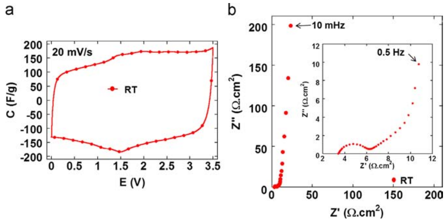
Figure 3 Room temperature electrochemical characterization of a-MEGO electrodes in (\text{PIP}_{13}\text{-FSI})_{0.5}(\text{PYR}_{14}\text{-FSI})_{0.5} electrolyte: CVs collected at 20 mV/s with the electrochemical window of 3.5 V and showing capacitance of 150 F/g (a) and the corresponding EIS Nyquist plot (b). Inset in (b) shows data at the high-frequency range.
