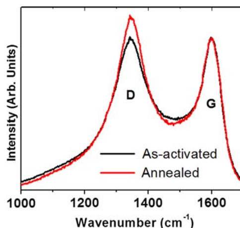
Figure 2 Raman spectra of as-a-MEGO in the carbon spectral range showing the bands corresponding to disordered structures (D) around 1350 \text{ cm}^{-1} and in-plane vibrations of graphite (G) around 1600 \text{ cm}^{-1} . Note that there is no significant change of the structure as a result of annealing.
