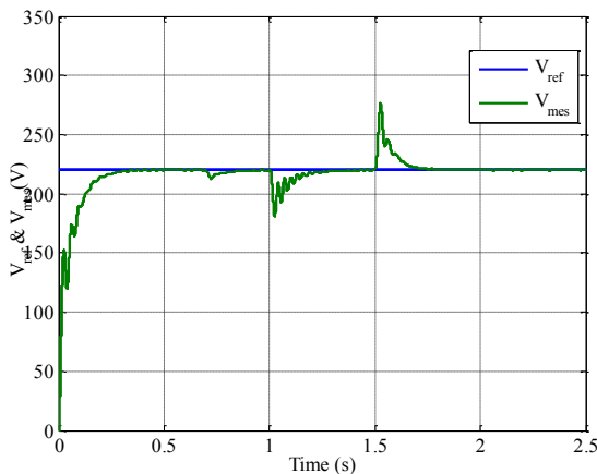
Fig. 3. The peak value of the PW phase voltage and its reference.
