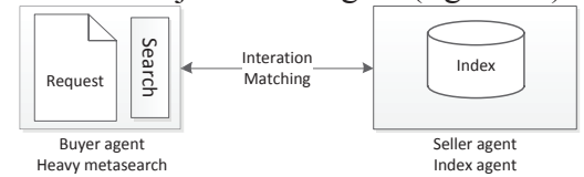
Fig. 11. Heavy metasearch and index agents
