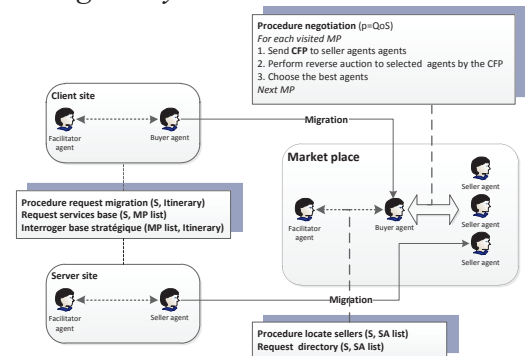
Fig. 3. The SB multi-agents system
