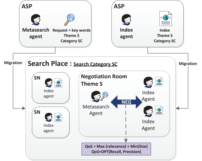
Fig. 12. Overview of MP-IR architecture
