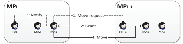
Fig. 8. The global migration of agents
