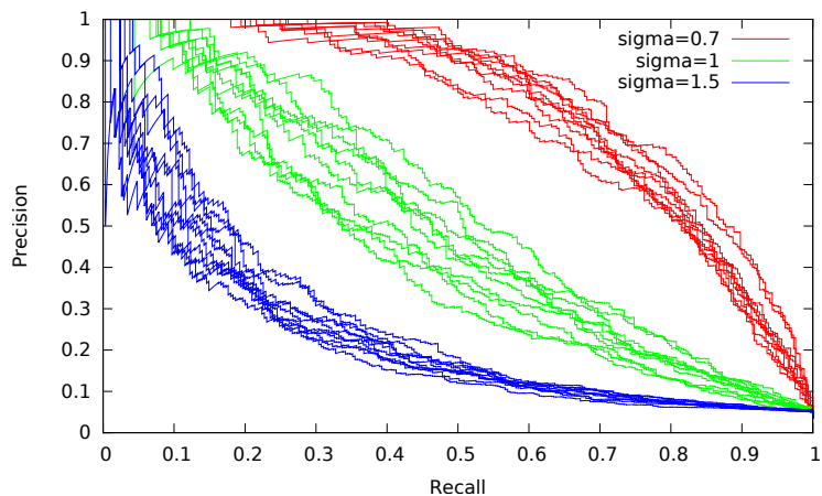
Figure 3 Influence of \sigma . PR curves for simulations with varying \sigma , with means (\mu_-, \mu_0, \mu_+) = (-1, 0, 1) . Ten simulations are run for each value
