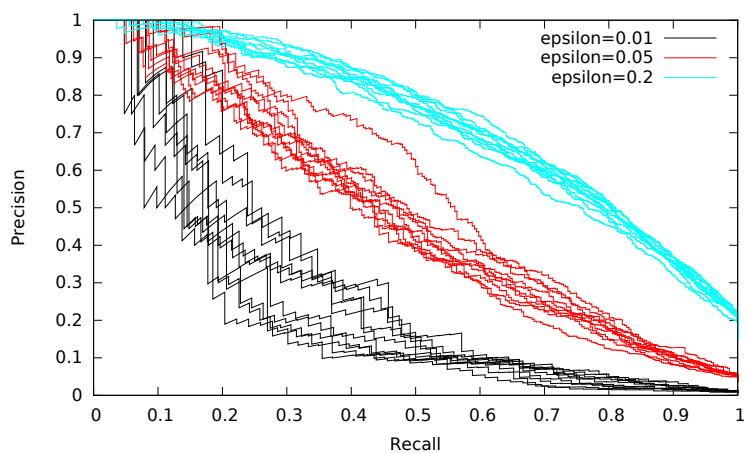
Figure 4 Influence of \epsilon . PR curves for simulations with varying \epsilon . Ten simulations are run for each value
