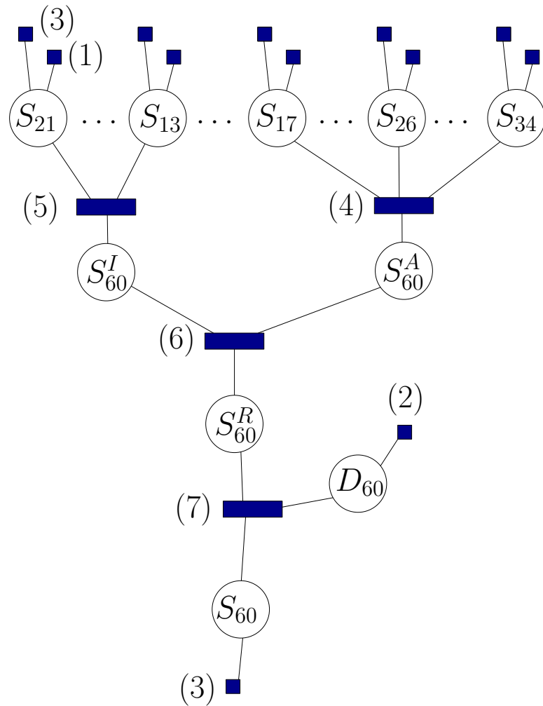
Figure 2 A partial view of the factor graph. The factor graph corresponding to Figure 1. The squares correspond to the factors, and are numbered according to the text. The algorithm iteratively updates the distribution of the circled variables.
