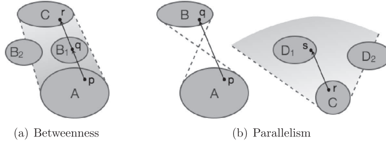
Fig. 2. Modelling betweenness and parallelism between regions.
