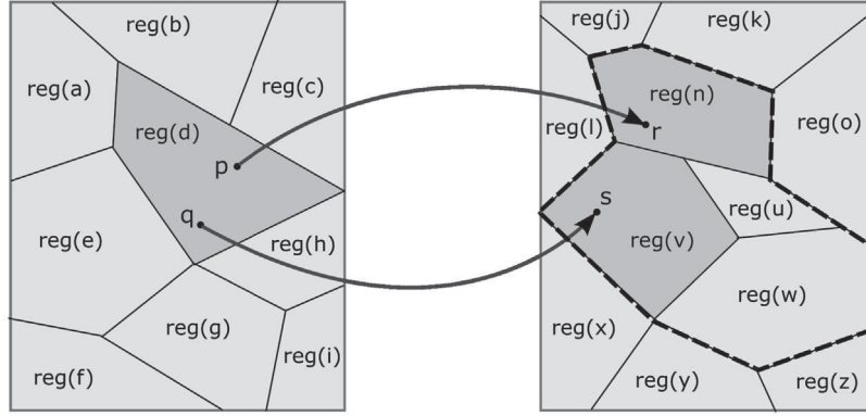
Fig. 5. Mappings from \mathfrak{B} (left) to \mathfrak{C} (right).
