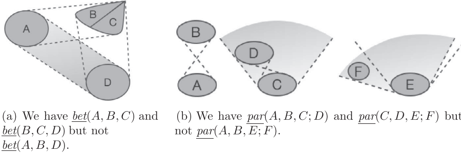
Fig. 3. The relations \underline{bet} and \underline{par} are not transitive.
