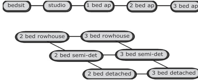
Fig. 4. Qualitative description of a conceptual space of housing types.
