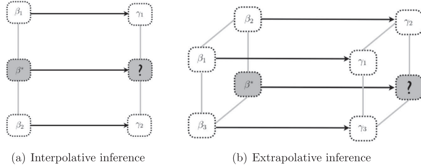
Fig. 1. Modelling betweenness and parallelism between regions.
