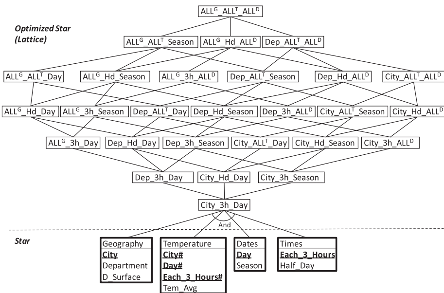
Figure 4. Classical lattice.
