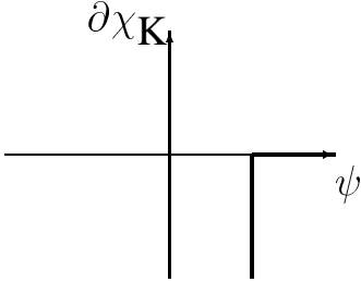
Figure 2.2. Graph of \partial\chi_{\mathbf{K}}
