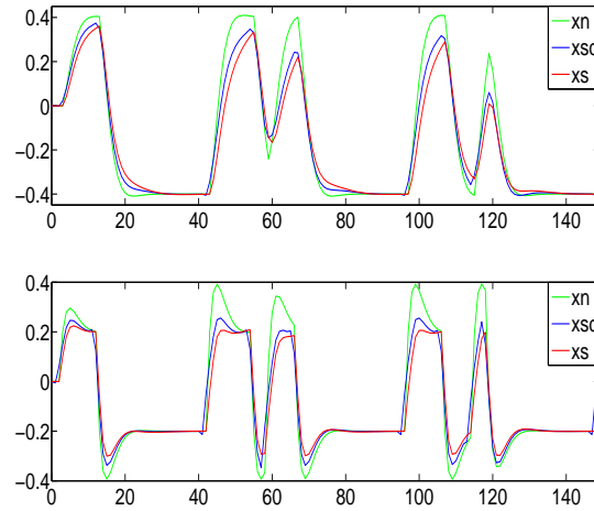
Figure 7: System states
