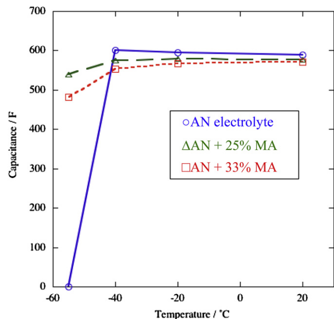
Fig. 4. Evaluated capacitance from discharge curves for 1 M TEABF 4 in (○) AN, (Δ) AN + MA (75:25) and (□) AN + MA (67:33) at +20, -20, -40 and -55 °C.
