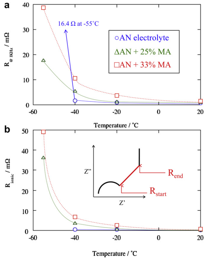
Fig. 6. (a) change of resistance at 1 kHz ( R_{@1kHz} ) with temperature and (b) ionic resistance in carbon pores estimated from EIS results for 1 M TEABF 4 in (○) AN, (△) AN + MA (75:25) and (□) AN + MA (67:33) at +20, -20, -40 and -55 °C.
