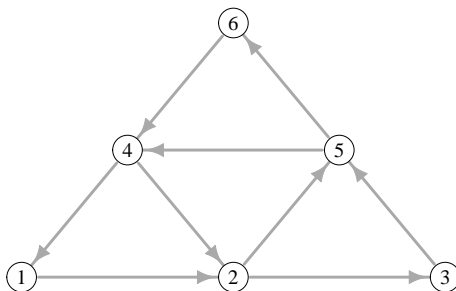
Figure 8: Two simple cycles with three common vertices.
