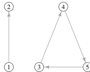
Figure 2: The self-avoiding hike h = \omega_{12}\omega_{34}\omega_{45}\omega_{53} from v_1 to v_2 contains n(h) = 2 connected components: the path \omega_{12} and the cycle \omega_{34}\omega_{45}\omega_{53} .
