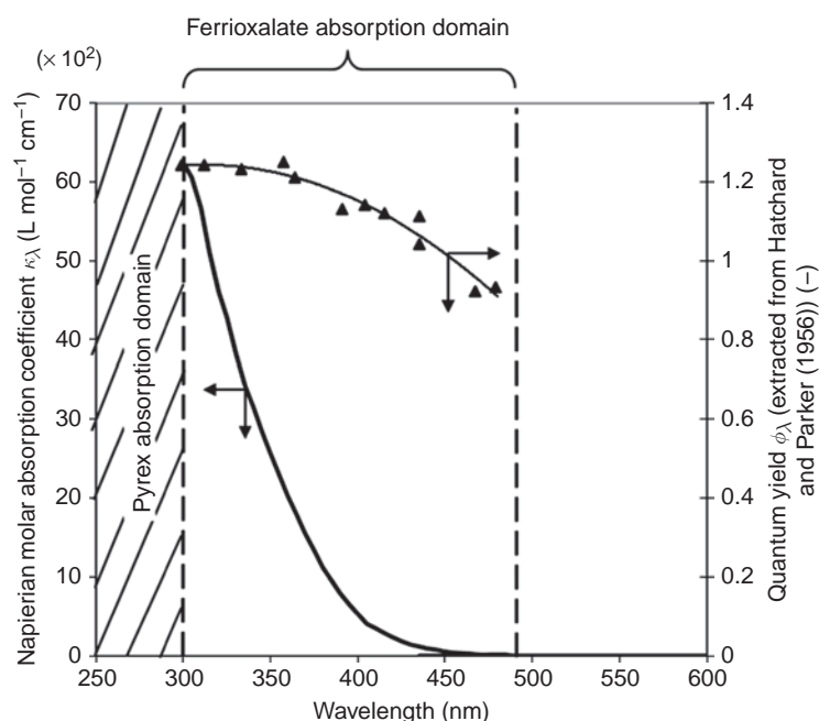
Figure 3 Dependence of the actinometer properties on the wavelength (Napierian molar absorption coefficient, quantum yield)
