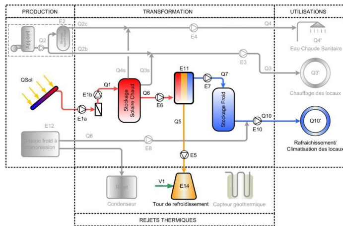
Fig. 1. PISTACHE cooling mode configuration (RAFSOL)
