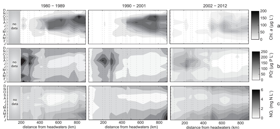
Figure 3. Spatiotemporal diagrams of monthly median levels of Chl a (a), \text{PO}_4^{3-} (b) and \text{NO}_3^- (c) during three periods along a longitudinal profile. Dotted vertical lines correspond to the monitoring stations (Fig. 1).
