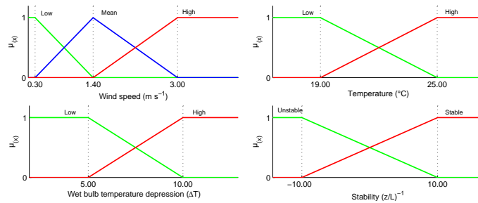
Figure 6: Fuzzy input partitions for pesticide loss data
