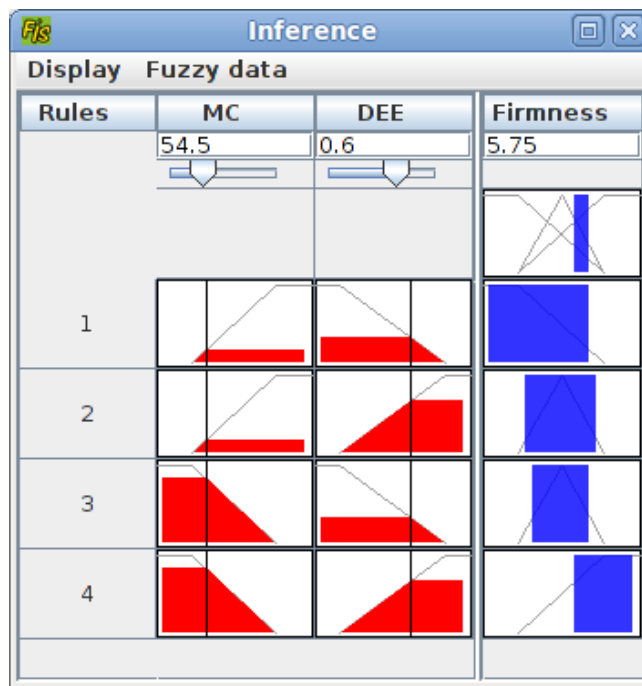
Figure 11: Firmness inference with implicative rules and a precise value
