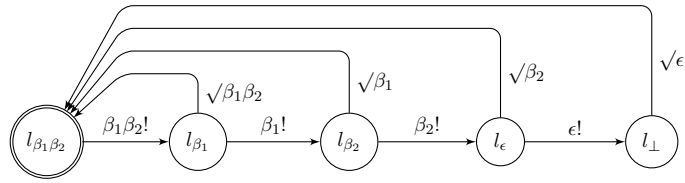
Figure 8. The shape of timed automaton TA_\surd for B^\otimes = \{\beta_1\beta_2, \beta_1, \beta_2, \epsilon\} , where \sqrt{\beta_1\beta_2} , \sqrt{\beta_1} , \sqrt{\beta_2} , \sqrt{\epsilon} are all synchronous urgent communication labels.
