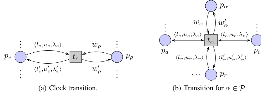
Fig. 2. Scheme of Petri net modelling of ANDy.
