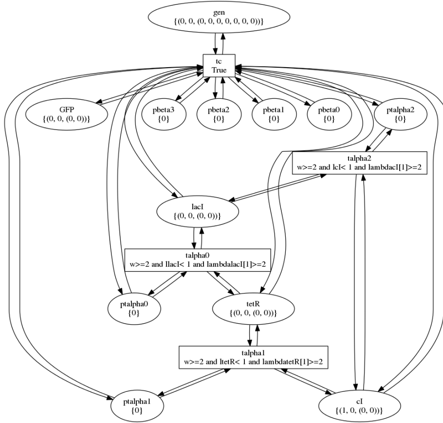
Fig. 3. The general shape of the ANDy network for the Repressilator from Example 1 (arcs annotations are omitted).
