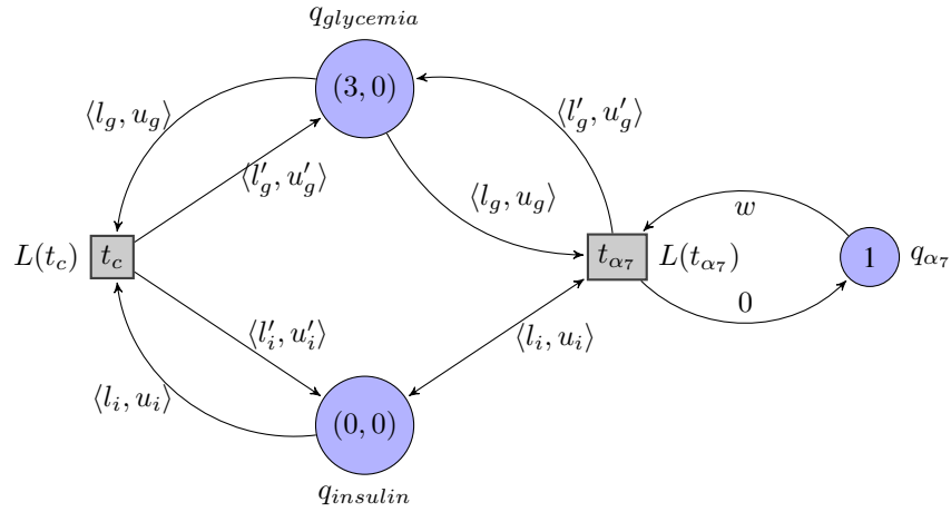
Fig. 8. A portion of the ANDy network of glucose metabolism with an initial marking.
