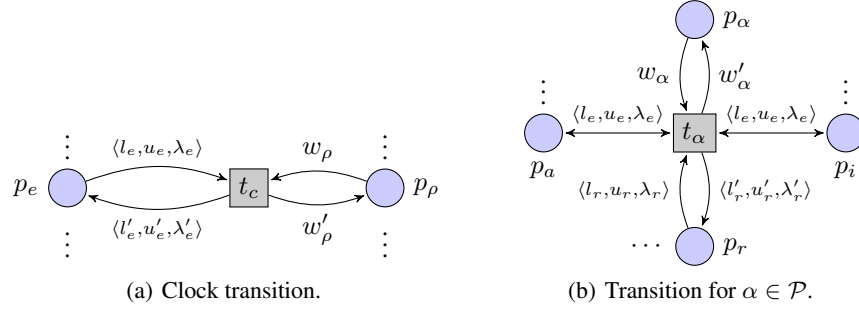
Fig. 2. Scheme of Petri net modelling of ANDy.
