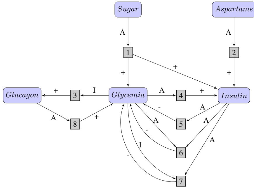
Fig. 7. Simplified ANDy network of glucose metabolism.
