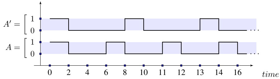
Fig. 4. Entities levels evolving with time corresponding to the given scenario.
