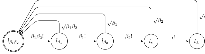
Fig. 5. The shape of timed automaton TA_{\surd} for B^{\otimes} = \{\beta_1\beta_2, \beta_1, \beta_2, \epsilon\} , where \sqrt{\beta_1\beta_2} , \sqrt{\beta_1} , \sqrt{\beta_2} , \sqrt{\epsilon} are all synchronous urgent communication labels.
