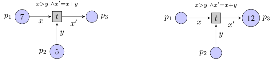
Fig. 1. Example of firing of transition t with \sigma = \{x = 7, y = 5, x' = 12\} .
