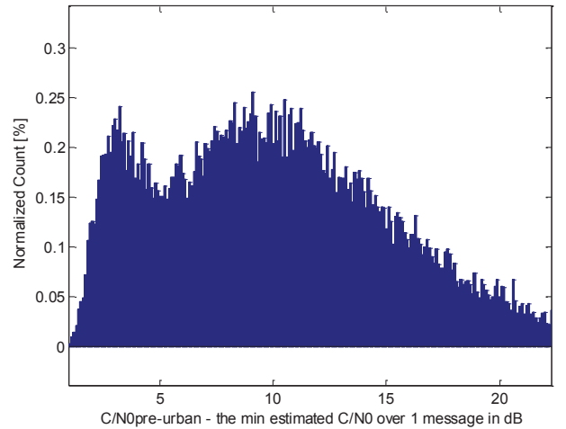
Figure 13: Distribution of the degradation between the C_{pre-urban}/N_0 value and the minimum estimated received C/N_0 over 1 message, for C_{pre-urban}/N_0 = 25 dB-Hz and ideal phase estimation with the DLR model
