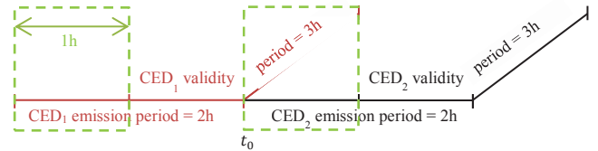
Figure 11: CED emission and validity periods diagram for GPS L1C
