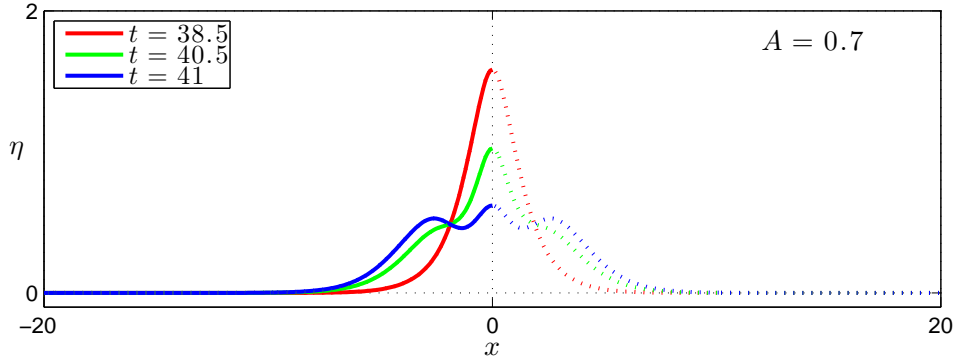
FIGURE 7. Reflection of solitary waves of normalized amplitude A = 0.7 at a vertical wall located at x = 0 , plotted together with the head-on collision of two solitary waves of the same amplitude to show their equivalence.
