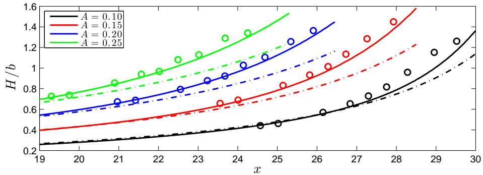
FIGURE 5. Comparison of the computed relative wave height H/b with experimental data of [GSSV94] for the shoaling of solitary waves on a plane beach of slope 1 : 35, and with Green's law. '—': Numerical solutions, 'o': Experimental data, '---': Green's law for Boussinesq systems
