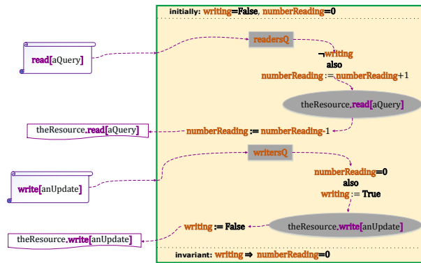
Swiss Cheese in the Actor Model [24]
