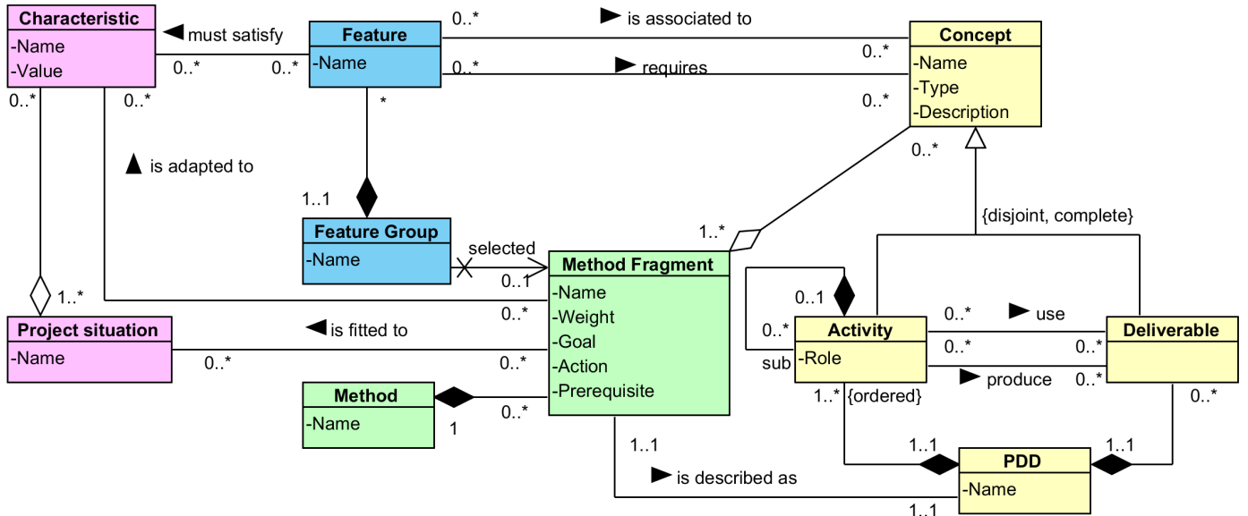
Fig. 2. Method Association concepts as a metamodel.
