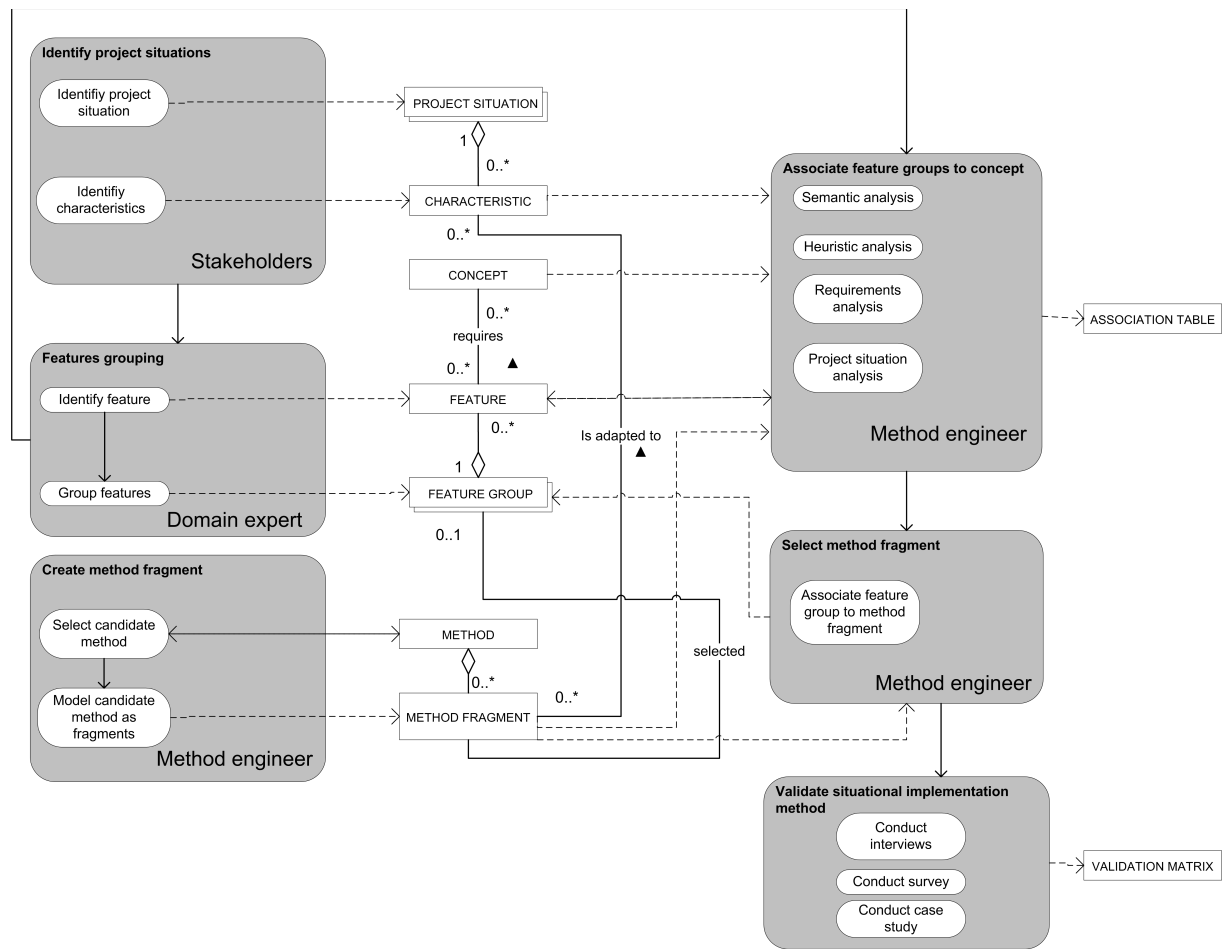
Fig. 3. PDD of the proposed approach.
