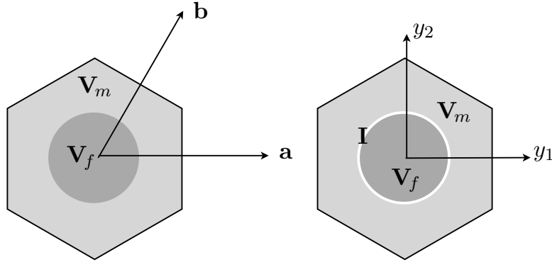
FIGURE 2. The case when the cell is a regular hexagon (left: bonded, right : debonded)
