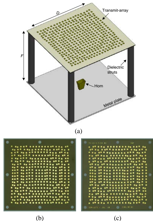
Fig.1 Perspective view of the transmit-array antenna (a), top view (b) and bottom view (c) photographs of the broadside-beam transmit-array.
