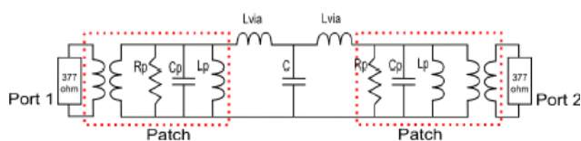
Fig. 5: Equivalent electrical model of the unit-cell.
