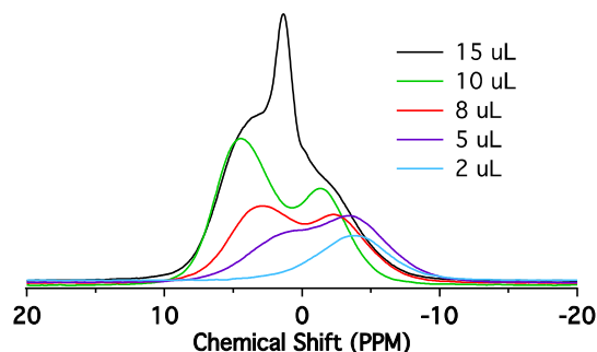
Figure 1. 11 B NMR spectra of YP-17 carbon films with different amounts of 1.5M TEA-BF 4 in acetonitrile in plastic bags.
