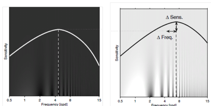
Figure 12: Contrast sensitivity function (CSF) of the human eye in dark (left) and bright (right) viewing conditions. Arrows labeled as \Delta \text{Sens.} and \Delta \text{Freq.} denote the amount of difference in magnitude and frequency of the peak sensitivity between the dark and bright cases. The figure is reproduced from [38].
