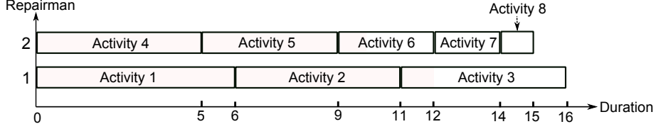
Figure 4: Optimal scheduling of 8 maintenance activities under 2 repairmen
