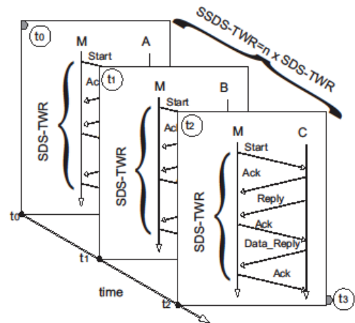
Figure 3. Ranging protocol SSDS-TWR
