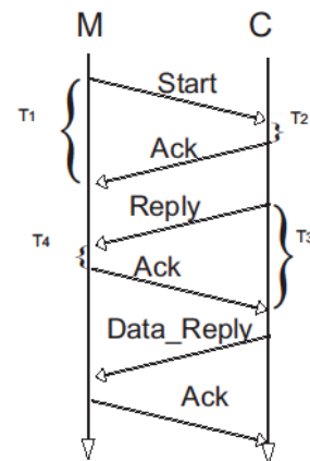
Figure 1. SDS-TWR protocol
