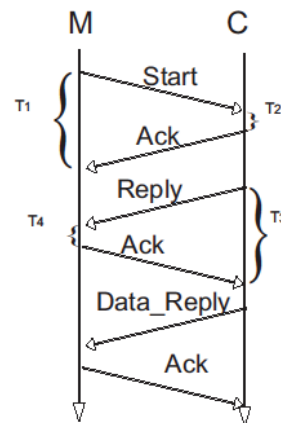
Figure 1. SDS-TWR protocol
