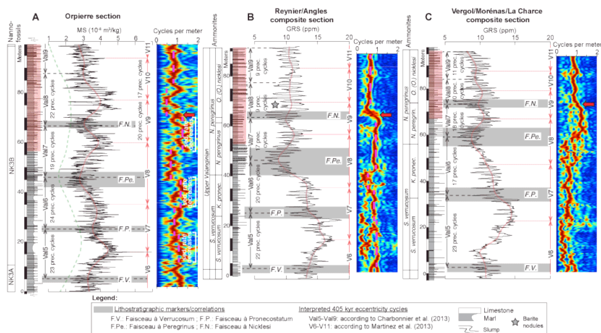
Figure 2: Cyclostratigraphic correlation of the Late Valanginian sections (SE France), and evulsive harmonic analysis (EHA) of the detrended physical proxy data (Val5 to Val9 cycles attributed to the 405 kyr eccentricity are removed) to describe variations in sedimentation rate, expressed through the change in thickness of couplets (i.e., wavelength of precession cycles). (A) Magnetic susceptibility (MS) variations at Orpierre section (from Charbonnier et al., 2013). 12% and 30% weighted averages of the series are shown (solid and dashed curves, respectively). (B) Gamma-ray spectrometry (GRS) variations at the Reynier and Angles (RA) composite section (from Martinez et al., 2013). (C) GRS variations at the Vergol, Morénas and La Charce (VMC) composite section (from Martinez et al., 2013). A 10% weighted average of the series is shown for RA and VMC (orange line). Note that all lithostratigraphic markers, and the 405 kyr cycles V6 to V11 in the RA and VMC sections are placed according to Martinez et al. (2013) (their figure 5). The orange shaded intervals in the three stratigraphic columns, encompassing V9, V10 and V11, correspond to those in which Martinez et al., 2013 have interpreted the couplets as being related to obliquity. Numbers of precession cycles within each 405 kyr cycle are also shown (see Figs. S2 to S4 for more details). The increase in sedimentation rate in the middle part of V9 cycle, which is pronounced in RA section, is indicated by red arrow in EHA spectrograms. Also, oscillations in sedimentation rate are indicated on the highly resolved Orpierre spectrogram.
