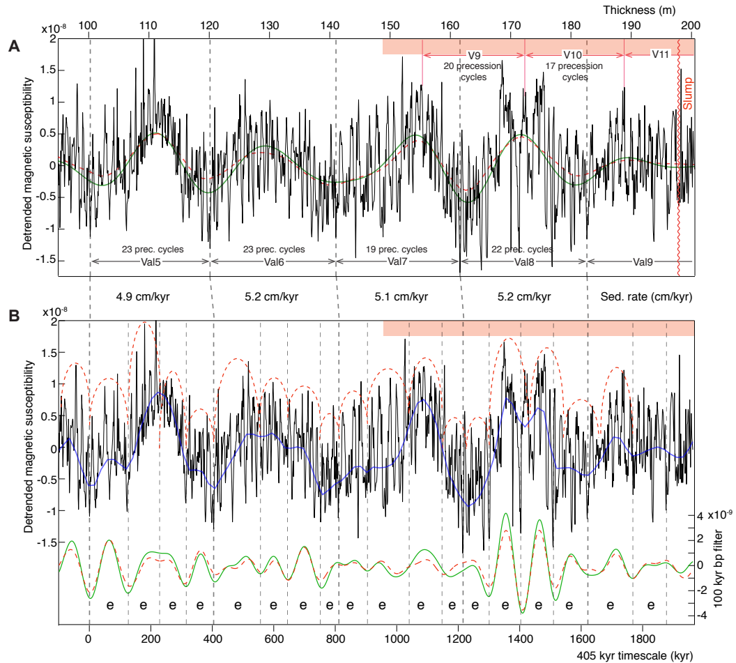
Figure 4: 405 kyr orbital tuning of magnetic susceptibility (MS) variations of the Late Valanginian interval at Orpierre section (meters as in Charbonnier et al., 2013; the lowermost ~3.25-m-thick marly interval associated to the slump is measured and added here to show how the MS signal is disturbed). (A) Untuned detrended MS data by subtracting a 30% weighted average of the series. A 12% weighted average fit of the already detrended (30% weighted average) series (solid line) and a gaussian bandpass filter ( 0.05 \pm 0.03 cycles/m, dashed line) are performed to highlight the interpreted 405 kyr eccentricity cycles Val5 to Val9 p.p. . Number of precession cycles within each 405 kyr cycle are also shown. V9, V10 and V11 are 405 kyr eccentricity cycles equivalent to those interpreted by Martinez et al. (2013) from Reynier/Angles and Vergol/Morénas/La Charce composite sections (see Fig. 2). The orange shaded interval encompassing V9, V10 and V11, corresponds to that in which Martinez et al. (2013) have interpreted the couplets as having an obliquity origin. (B) 405 kyr tuned MS. Weighted average smoothing (upper curve fit) and bandpass filtering ( 0.009 \pm 0.004 cycles/kyr, lower curve) are applied to the tuned MS data to show the short (100 kyr) eccentricity cycles (indicated by 'e'). Average sedimentation rates inferred from the 405 kyr tuning are also shown. Note that because of the high variability in MS amplitudes at the scale of couplets, it is difficult in several cases to capture boundaries of the short eccentricity cycles neither from filtering nor from smoothing techniques. For example, the middle Val5 cycle contains two amalgamated 'e' cycles not detected by smoothing, but slightly by filtering. Therefore, a possible interpretation from visual inspection is also proposed by dashed arcs.
