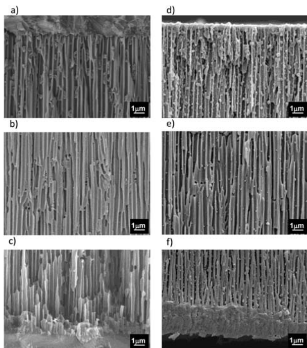
Fig. 1 FESEM images of the cross-section of CAAO membranes after solvothermal synthesis (left column) and static SBS MOF synthesis (12 cycles, right column). (a) and (d) correspond to views close to side A; (b) and (e) correspond to views of the cross-section central region; and (c) and (f) correspond to views close to side B. Complementary information is supplied by Fig. S2, S3 and S4, S5,† respectively.
