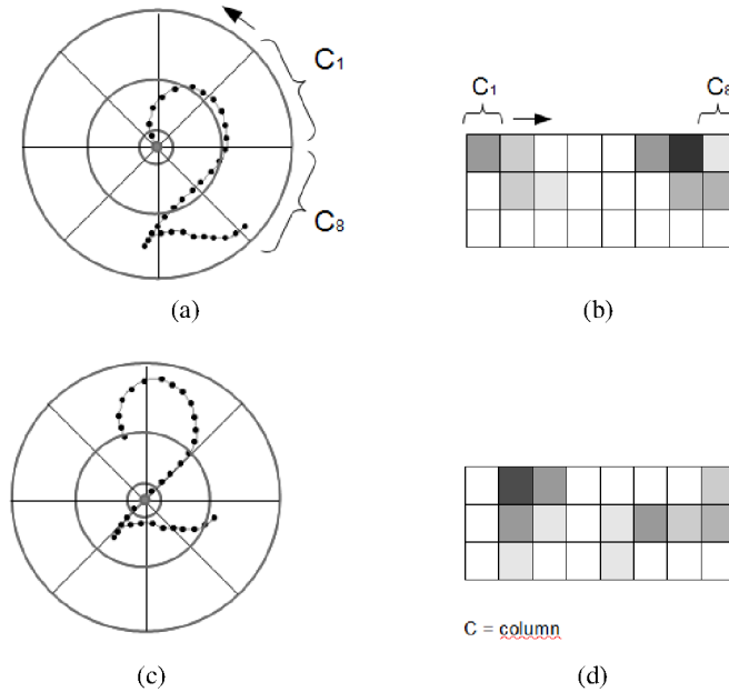
Figure 1. Shape context of two points of a symbol “2”: (a) and (c) show the sampled points and log polar histogram bins used to calculate shape context. (b) and (d) show the shape context histogram relative to (a) and (c) respectively. Dark cells mean higher values.
