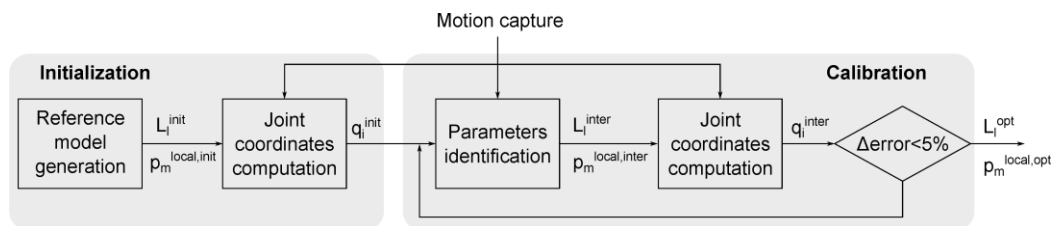
Figure 1: Calibration pipeline
