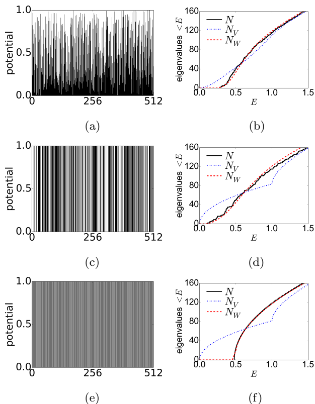
FIG. 3. (Left) Three different type of potentials: (a) random with uniform law on [0, 1] , (c) random Boolean (0 or 1), (e) periodic with 256 periods, V = 0 on the first half of the period, V = 1 on the second half. (Right) For each potential, the counting function N (solid black line) is represented, together with N_V (blue dash-dotted), Weyl's approximation using the original potential V (as defined in Eq. 11), and N_W (red dotted), the same with W . Notice in all cases the remarkable agreement between N and N_W .
