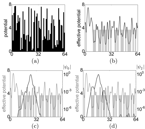
FIG. 1. (a) Random piecewise constant potential. (b) Effective confining potential W computed by solving Eq. 1 then taking the reciprocal of u . The wells of W are outlined in grey. (c) and (d) Probability density of the fundamental state |\psi_0\rangle of energy E_0 = 1.58 (resp., second excited state |\psi_2\rangle with E_2 = 1.62 ) in logarithmic scale superimposed on the effective potential W (light gray line). One can see that the decay of both eigenfunctions occurs mostly outside these wells, i.e., in the barriers of W , and stops inside these wells.
